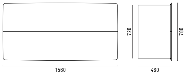
YSCT1A7FD1 Storage element 1560x780
