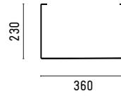
YSIS1A2 Metal shelf for 560x560 element
